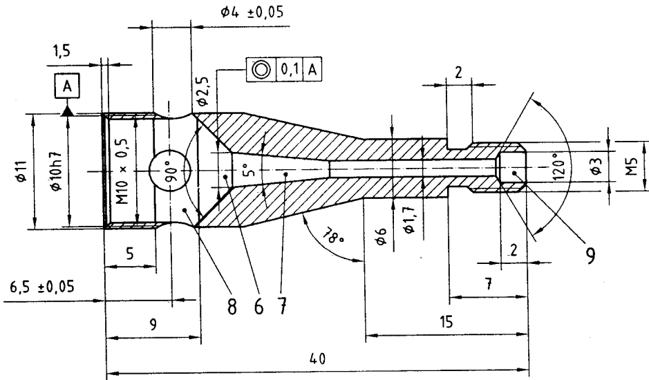
d) Burner tube
